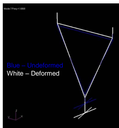
Figure 27: Mode 1: 1.69 Hz
