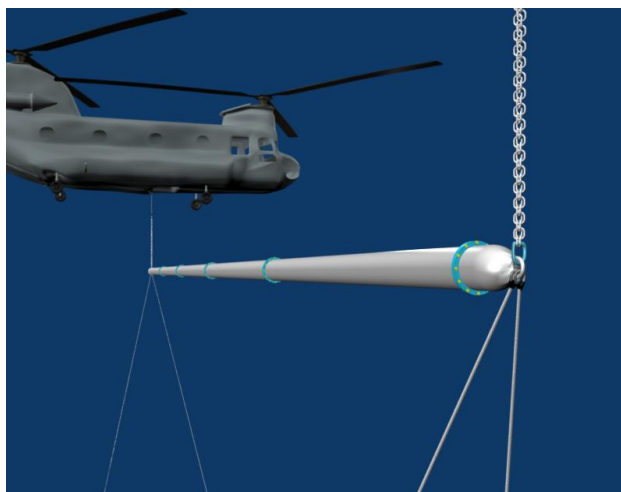
Figure 36: Spreader Bar Connections
