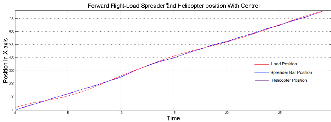
Figure 61: Forward Flight With Control Implemented
