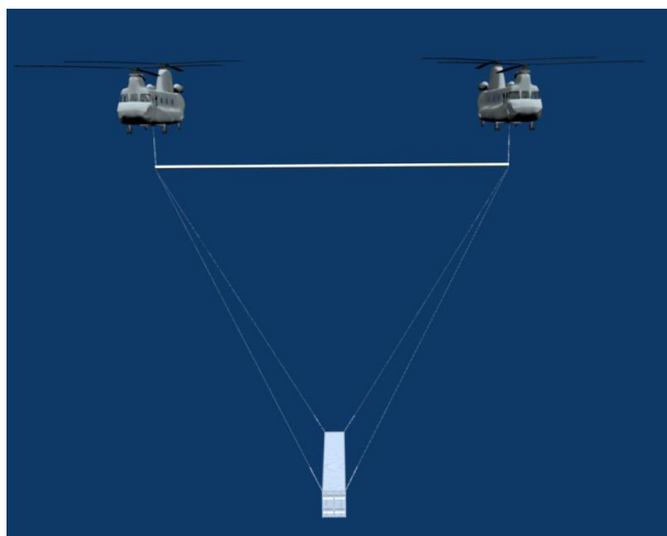
Figure 35: Twin-Lift System Configuration
