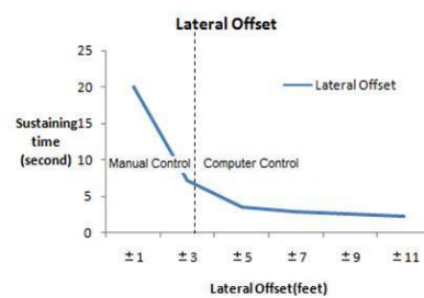
Figure 57: Lateral Offset
