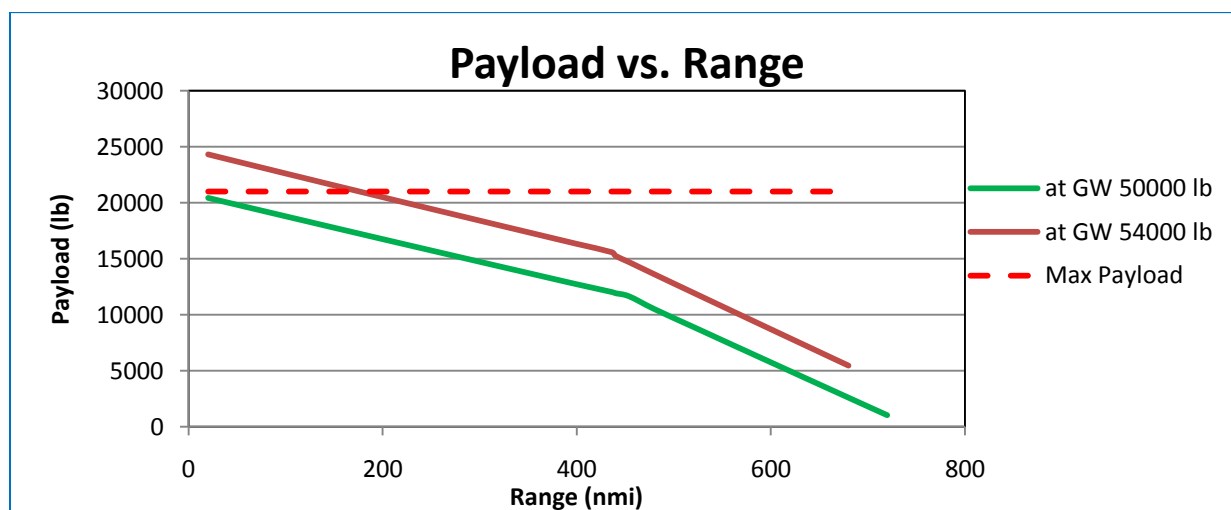
Figure 13: Payload-Range Diagram
