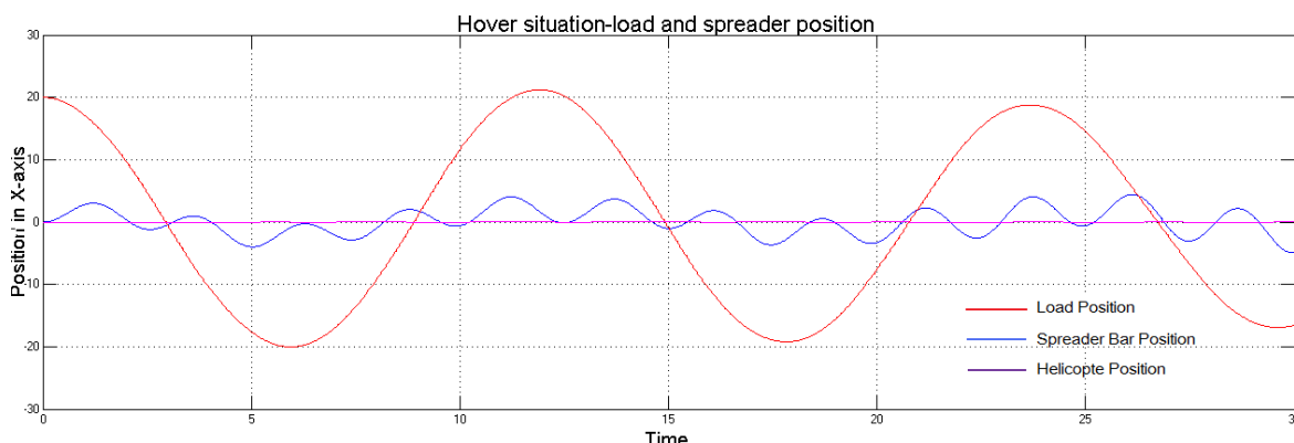
Figure 45: Load Oscillation
