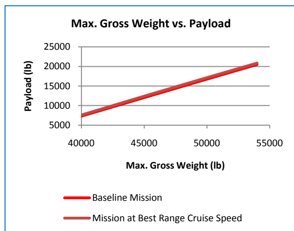
Figure 14: Max Payload Comparison at Different Flight Conditions
