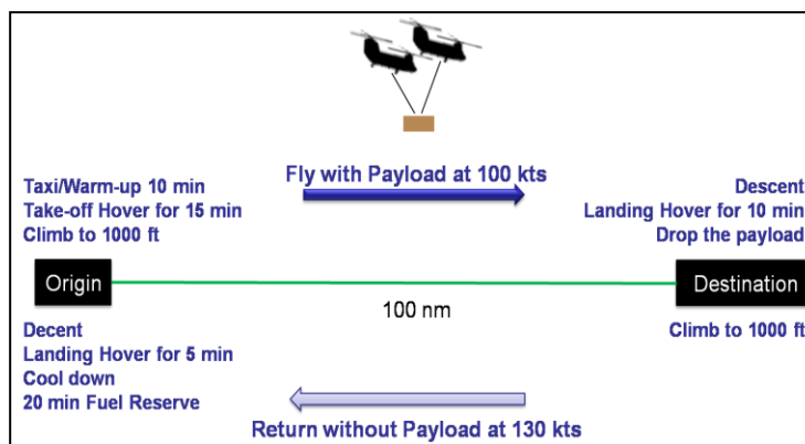
Figure 2: Mission Breakdown
