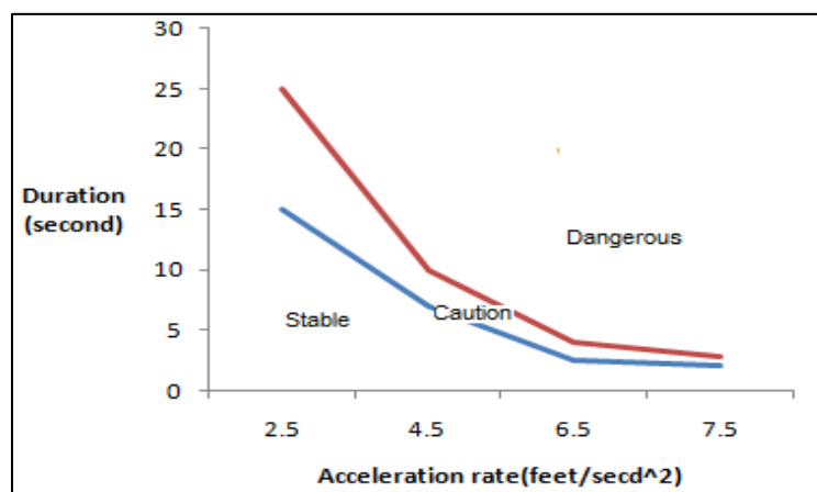
Figure 52: Operational Boundaries
