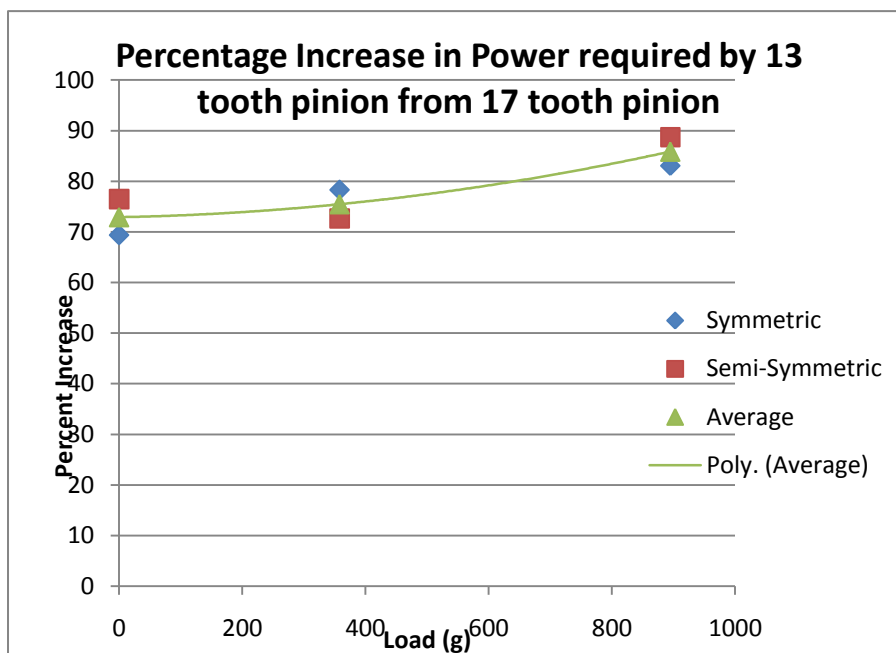
Figure 78: Percentage increase in power required by 13 tooth pinion from the 17 tooth pinion
