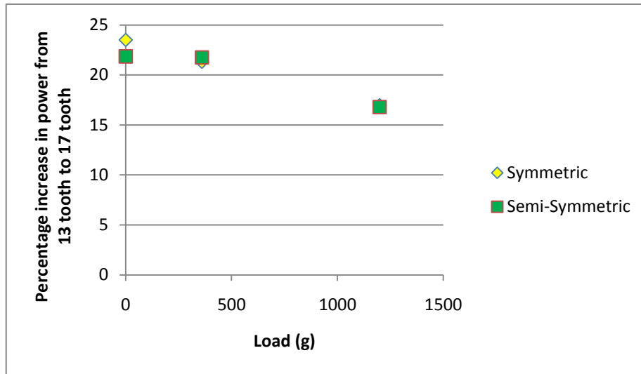
Figure 76: Pinion Change Plot
