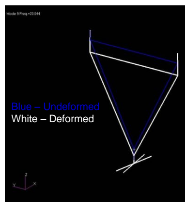
Figure 29: Mode 3: 20.04 Hz
