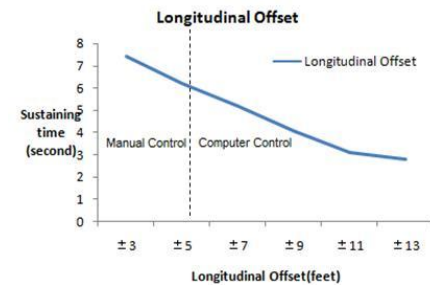
Figure 58: Longitudinal Offset
