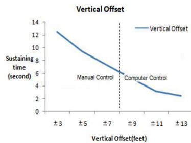
Figure 56: Vertical Offset
